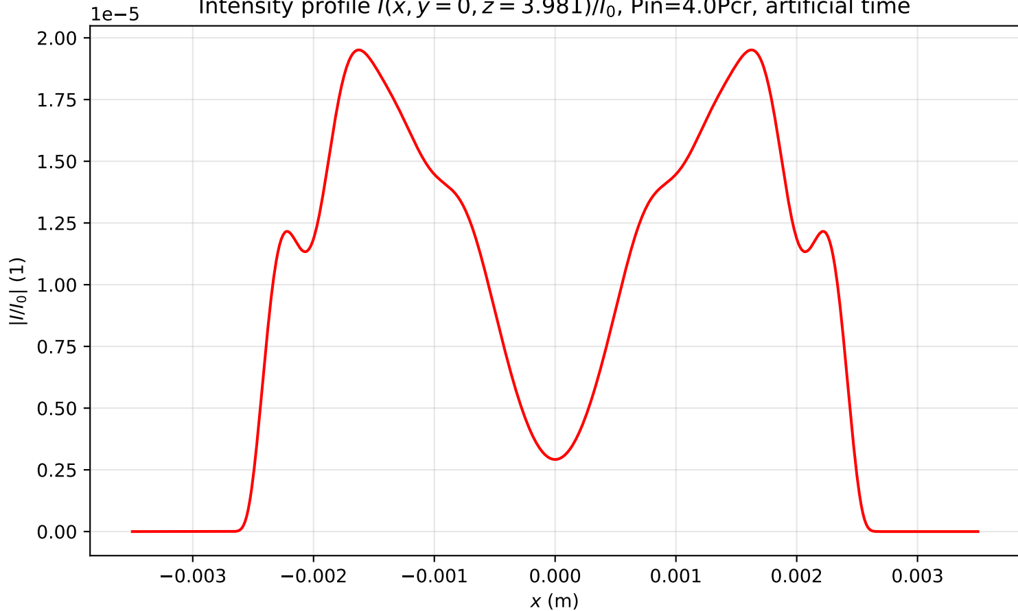
Intensity profile I(x, y = 0, z = 3.981)/I_0 , P_{in}=4.0P_{cr} , artificial time
